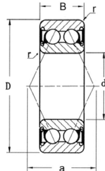
Type 2RS with two seals (non-contact)
