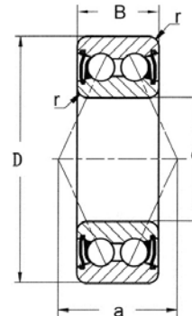
Type ZZ with two shields
